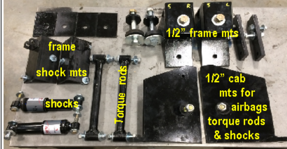
Bolt on "LEVEL RIDE" Tractor Cab AIR RIDE Kit
